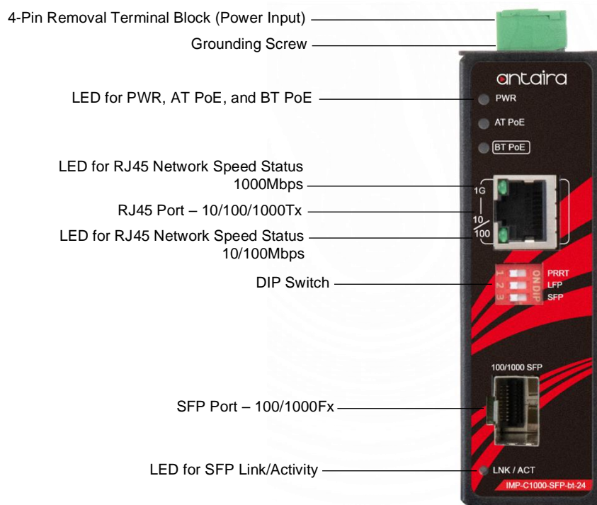
Figure 2.2 Front Panel
